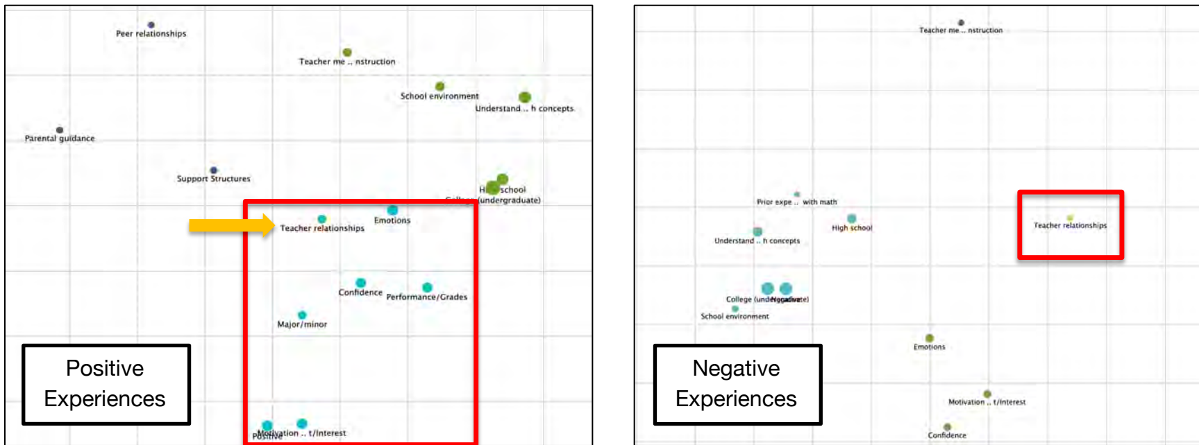
Figure 1 Code co-occurrence maps for positive (left panel) and negative (right panel) math learning experiences. Aspects of students' math learning experiences were clustered based on the frequency with which they intersected either with our negative or positive valence codes. Codes that co-occurred more frequently appear closer on the maps indicating that these aspects were discussed together more frequently in the same segments within and across focus groups. Distinct clusters are represented by different colors. Clusters were used to generate seven (three positive, four negative) overarching themes. Red boxes highlight our key finding that the teacher relationships code clusters with codes related to self-efficacy in positive math learning experiences, whereas it clusters alone in negative experiences. The orange arrow points to the mapping location of the teacher relationships code within the cluster.
